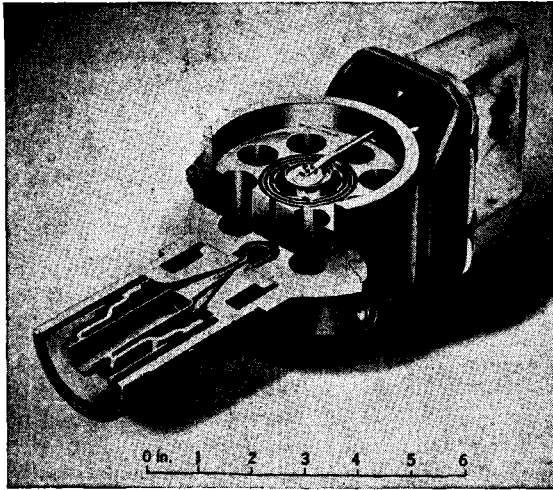
FIG. 5-1.—Center-loop coupling.
